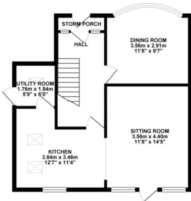
GROUND FLOOR 51.42 sq. m. ( 553.49 sq. ft. )
